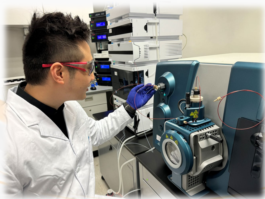
Analyses of pharmaceutical samples by liquid chromatograph-tandem mass spectrometer.
