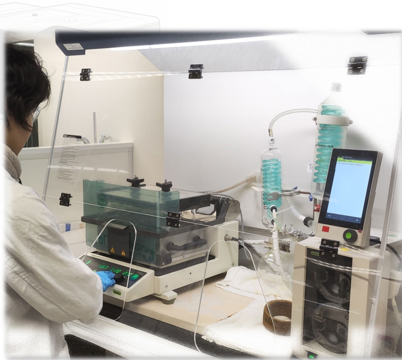
Analysis of total fat content in food samples by solvent evaporator.
