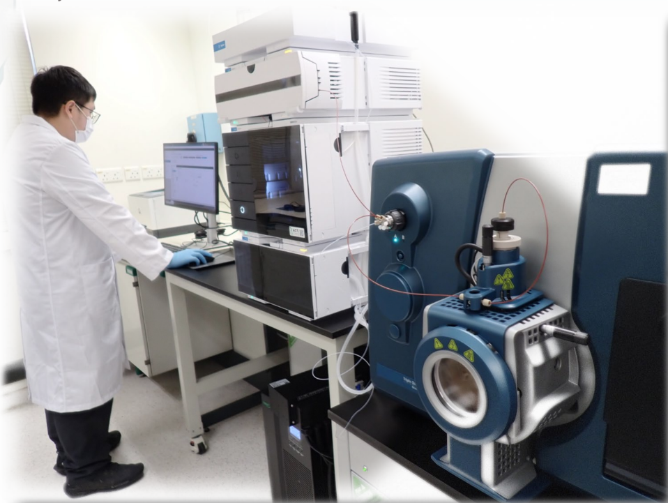
Liquid chromatography-mass spectrometry.
