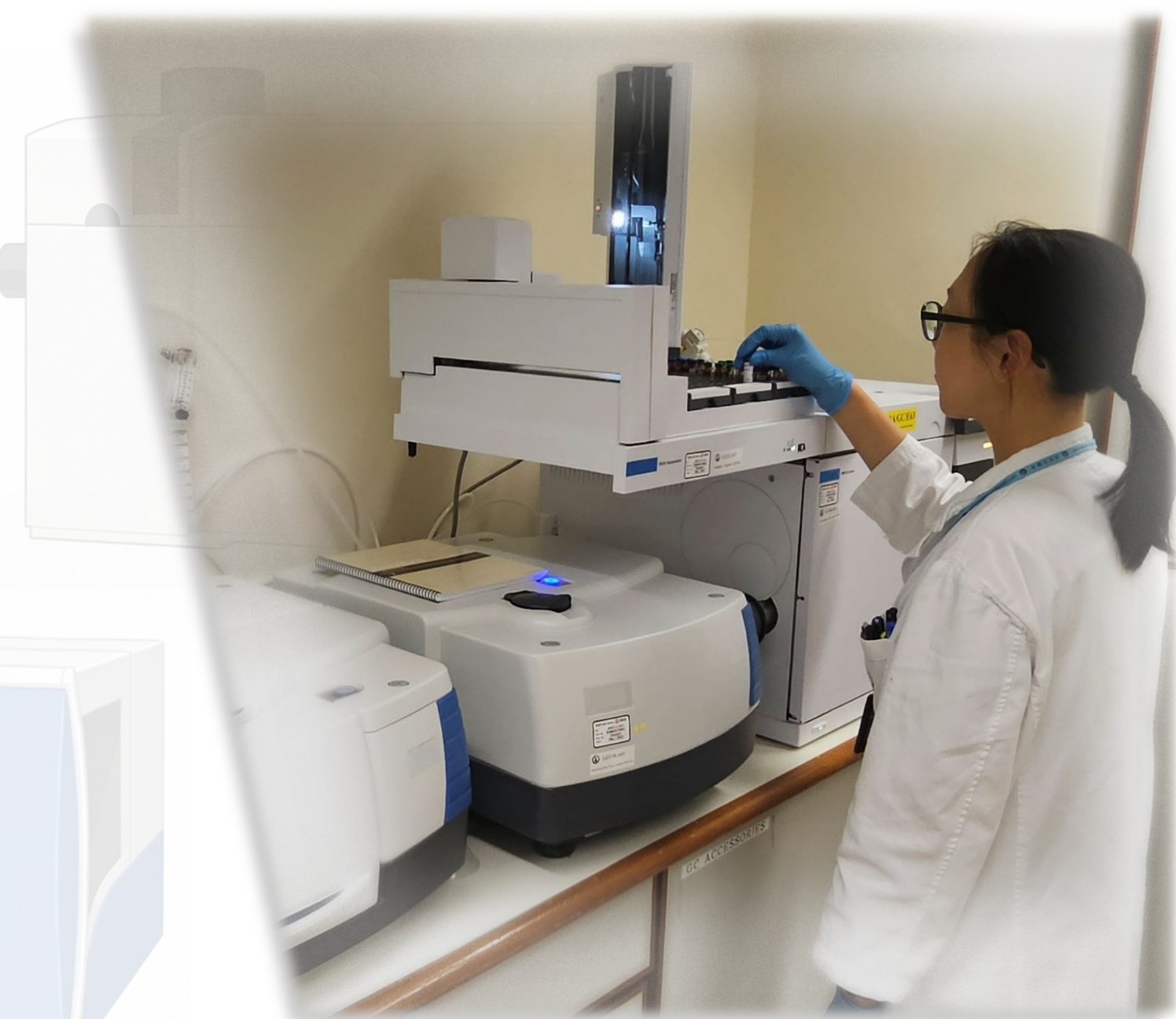
Analysis of ozone depleting substances (ODS) by gas chromatograph with Fourier transform infrared spectrometer system.
